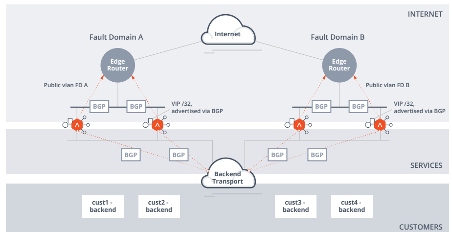
Figure 1: Application Deployment with Avi
