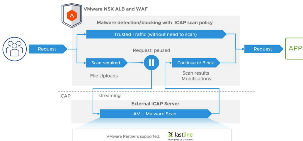
VMwareNSX ALB (Avi) and WAF – ICAP integration Architecture
